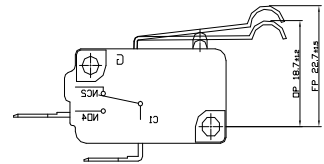
RS Lever
