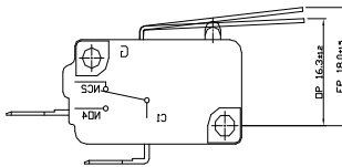
L Lever
